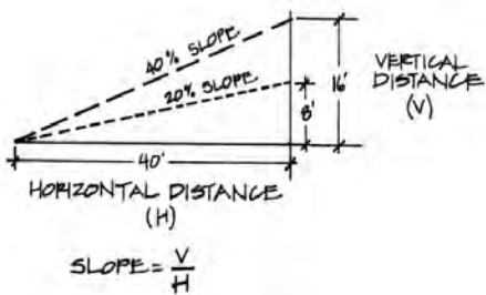
SLOPE CALCULATION
