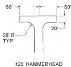
TURNAROUND DIMENSIONS
