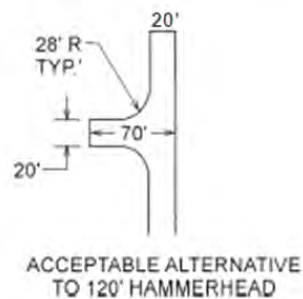
TURNAROUND DIMENSIONS
