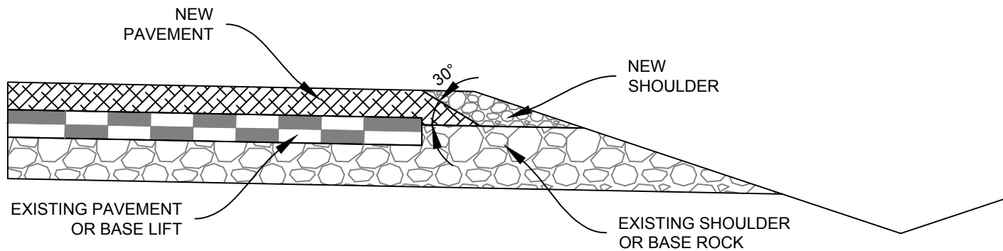
TYPICAL SECTION
